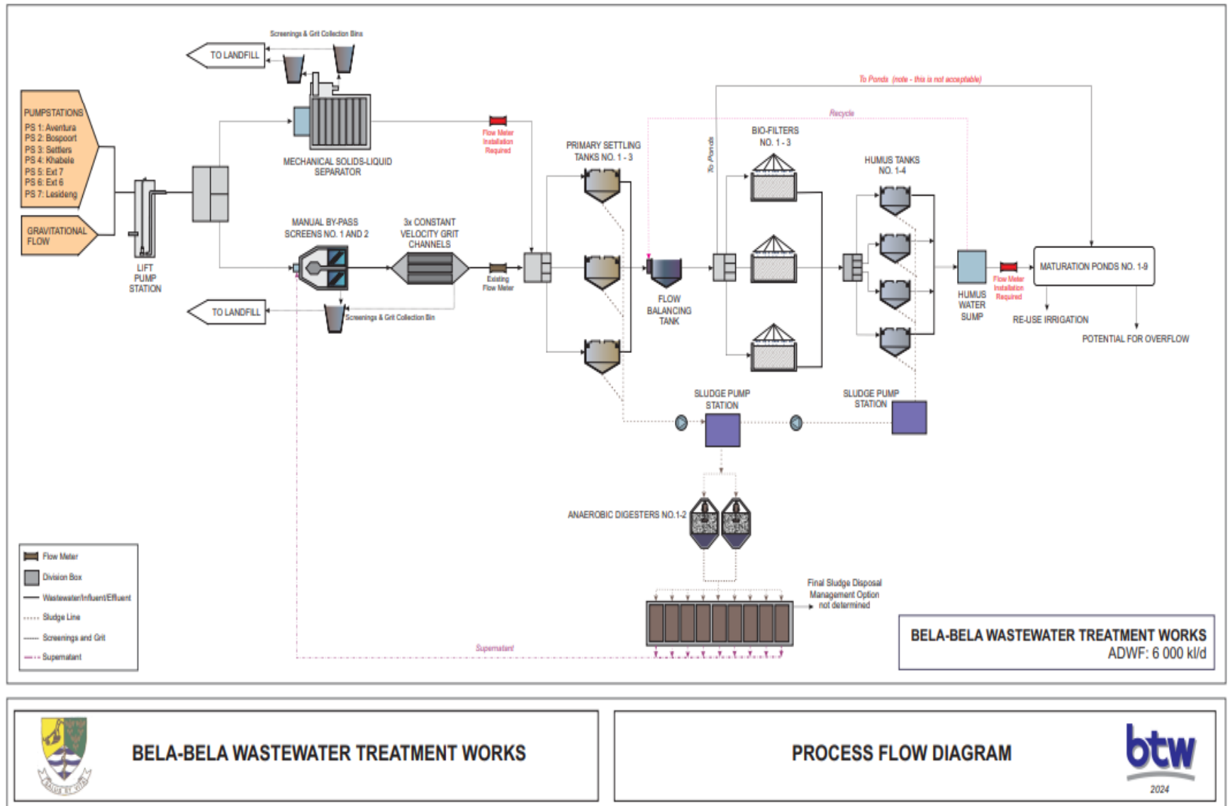
FIGURE 1: WARMBATHS WWTW – PROCESS FLOW DIAGRAM
