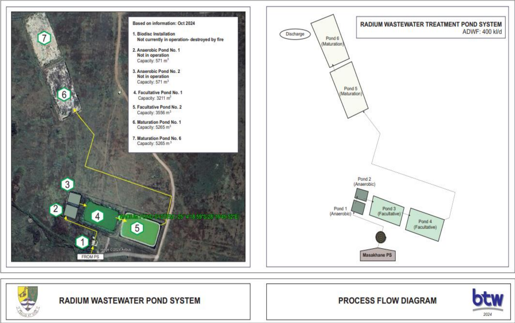
FIGURE 3: RADIUM/MASAKHANE POND SYSTEM – PROCESS FLOW DIAGRAM
