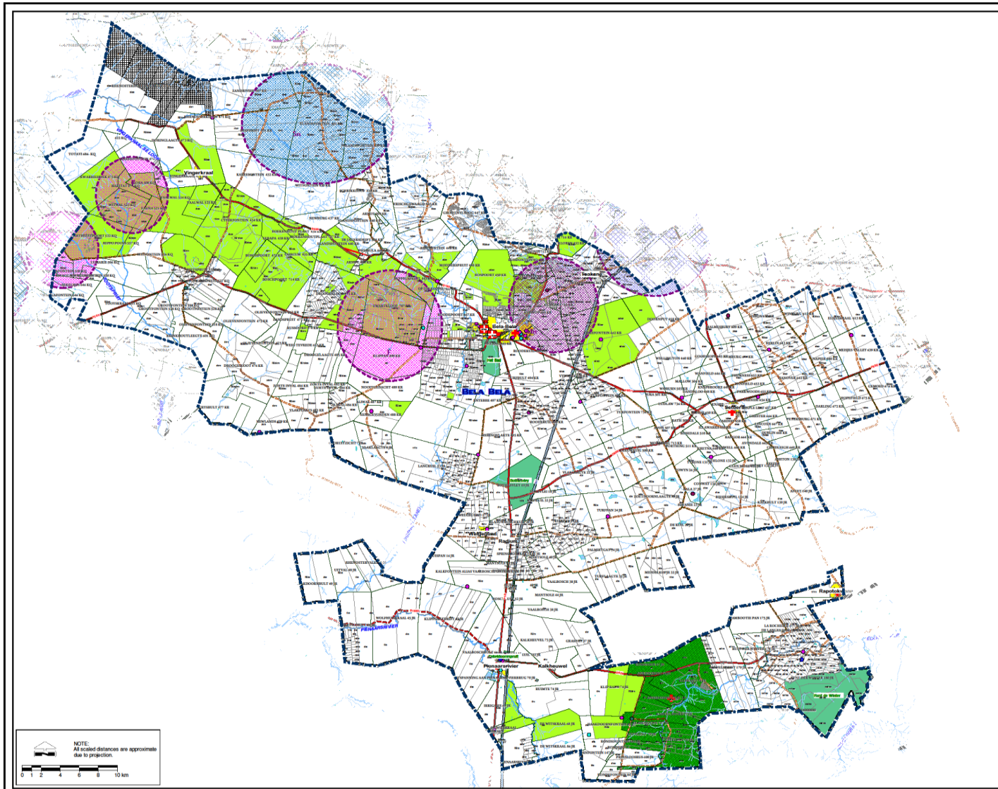
Figure 9: Depiction of Land Uses within Bela-Bela Municipality
