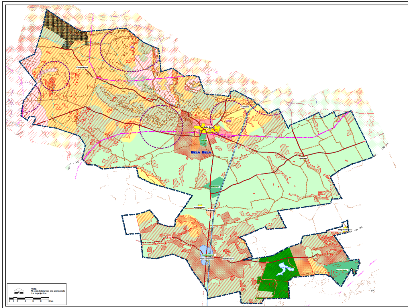
Figure 19: Environmentally Sensitive Areas
